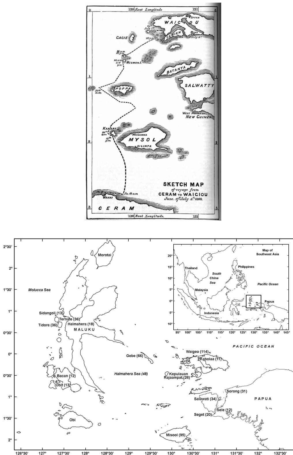
Figure 1. Maps depicting the study area; above: Wallace's voyage to Kepulauan Rajaampat in 1860; below: study area bounded by 2° North and 2° South between 127-132° East showing some of the place names (and number of observations in brackets) used in this analysis; the complete list of place names and number of observations available for the region is presented in Appendix A. Map drawn by A. Atanacio (Los Baños, Laguna, Philippines).
